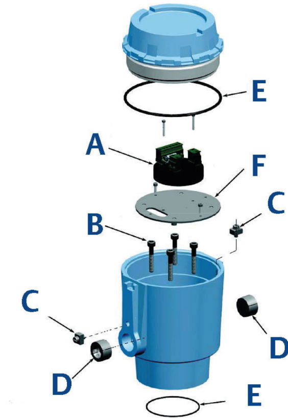
FIGURE 3: LOCAL MOUNTED ENCLOSURE (LME) WITH STANDARD DUAL-CHANNEL PREAMPLIFIER
