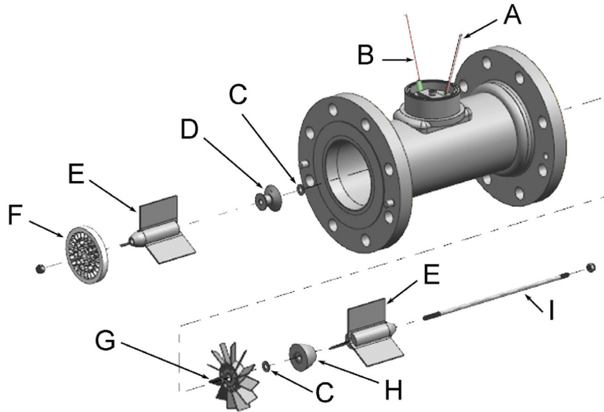
FIGURE 5: BLADE TYPE ROTOR EXPLODED VIEW
