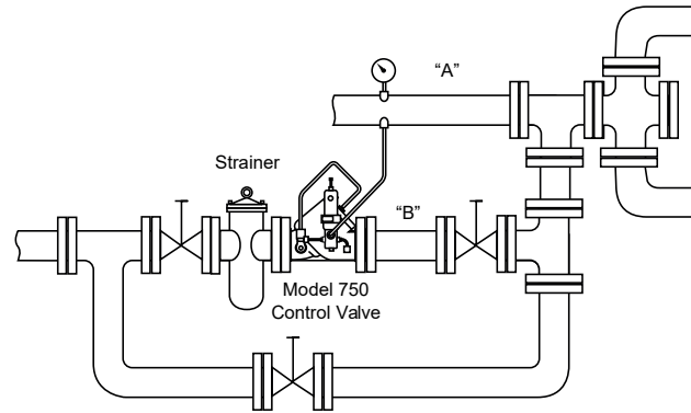
FIGURE 3 - PIPELINE "A" NORMALLY PROVIDES ALL THE PRODUCT FOR DISTRIBUTION UNLESS PRESSURE DROPS BELOW A REQUIRED MINIMUM. WHEN THIS OCCURS THE MODEL 750 INSTALLED IN AN AUXILIARY LINE "B" AND SENSED TO THE MAIN LINE "A", OPENS TO MAINTAIN PRESSURE AND FLOW UNTIL NORMAL MAIN LINE PRESSURE IS RESTORED.
