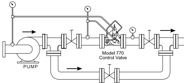
FIGURE 10 - THE MODEL 770 CONTROLS DIFFERENTIAL PRESSURE (LPG, NH3).
