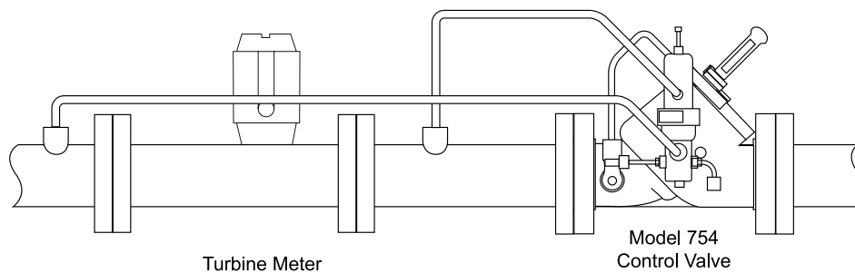
FIGURE 5 - MODEL 754 WITH TURBINE METER
