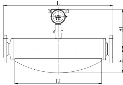
Compact version - Figure A.3.1 (Daniel® S-Type)
