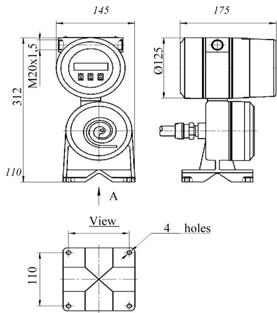
FIGURE A.4 OVERALL DIMENSIONS AND CONNECTION SIZE OF ELECTRONIC UNIT OF REMOTE TYPE
