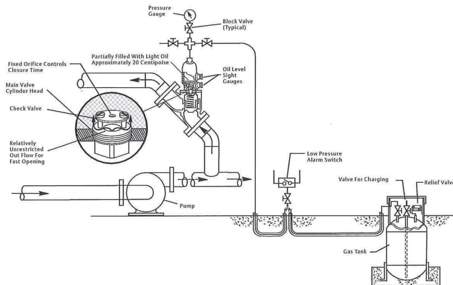
Figure 5-1: Typical installation - 766 Gas loaded pressure relief valve
