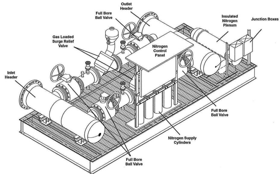
Figure 5-2: Surge relief system with nitrogen panel and plenum
