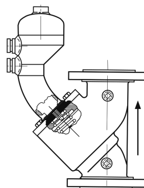
Daniel Surge Relief Valve for vertical installation
