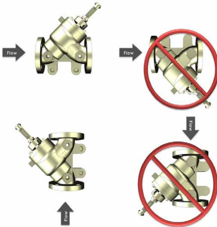
Figure 2-1: Valve orientation
